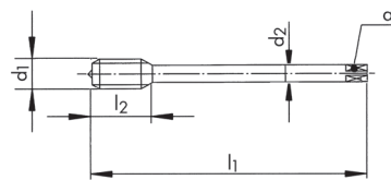
RTS462VS-3 (~DIN376)
