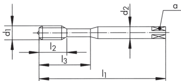
Q360VS-3 (DIN371)
